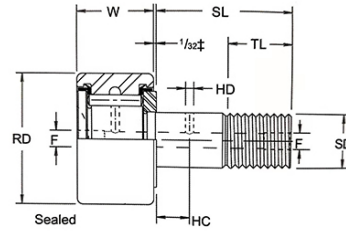
±1/16" on CF-5-S, CF-6-S, CF-7-S
